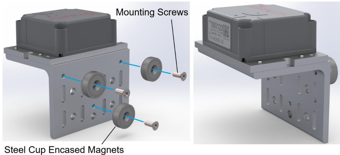
Figure 70: Installing Steel Cup Encased Magnets onto the Angle Bracket
