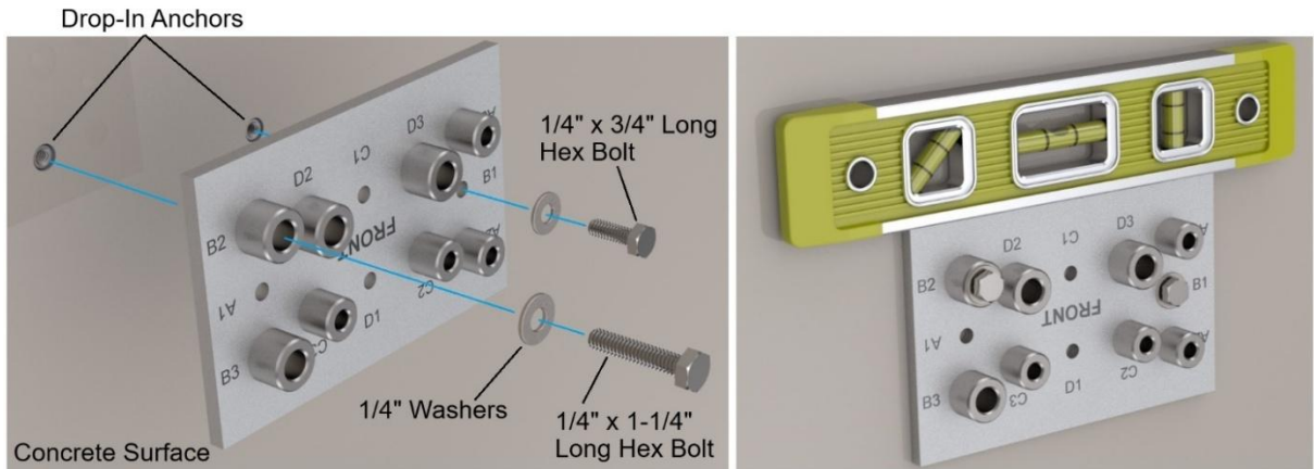
Figure 36: Leveling and Fastening Drilling Template on Hole B1 & Bushing B2 with \frac{1}{4} " Drop-In Anchors, Hex Bolts and Washers
