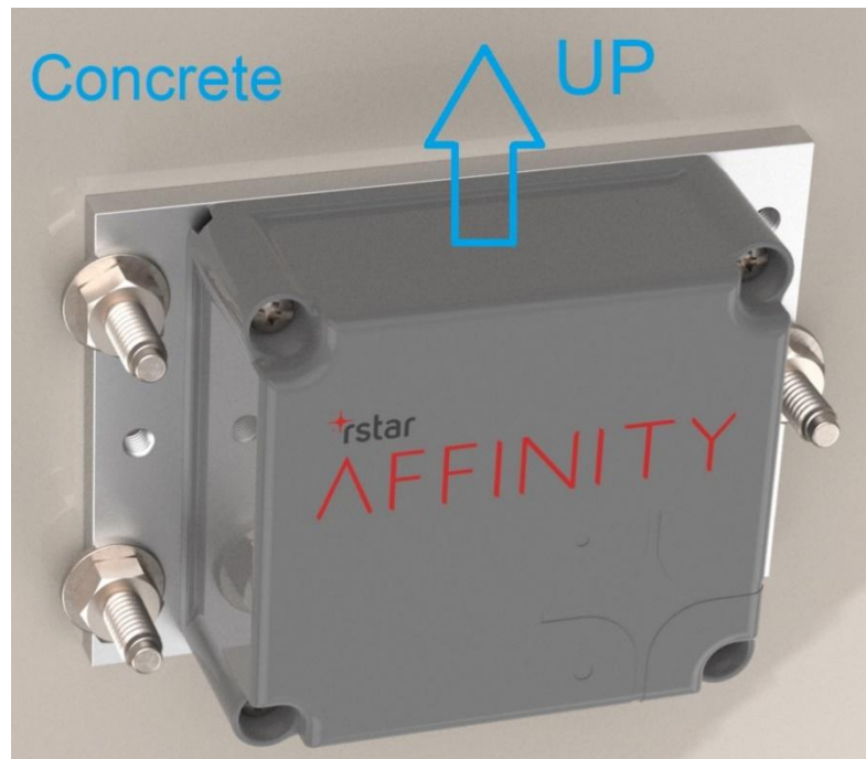
Figure 29: Direct Mounted Affinity Tilt Logger installed at Vertical Orientation using 1/4" Wedge Anchors
