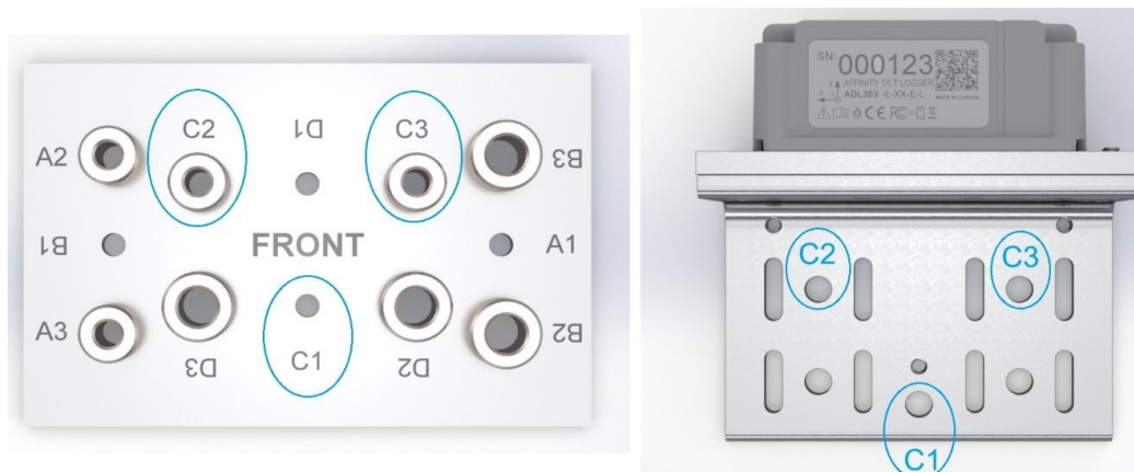
Figure 42: Drilling Template Hole Set C Corresponding to Tilt Logger Angle Bracket Mounting Holes for 1/4" Studed Wedge Anchor
