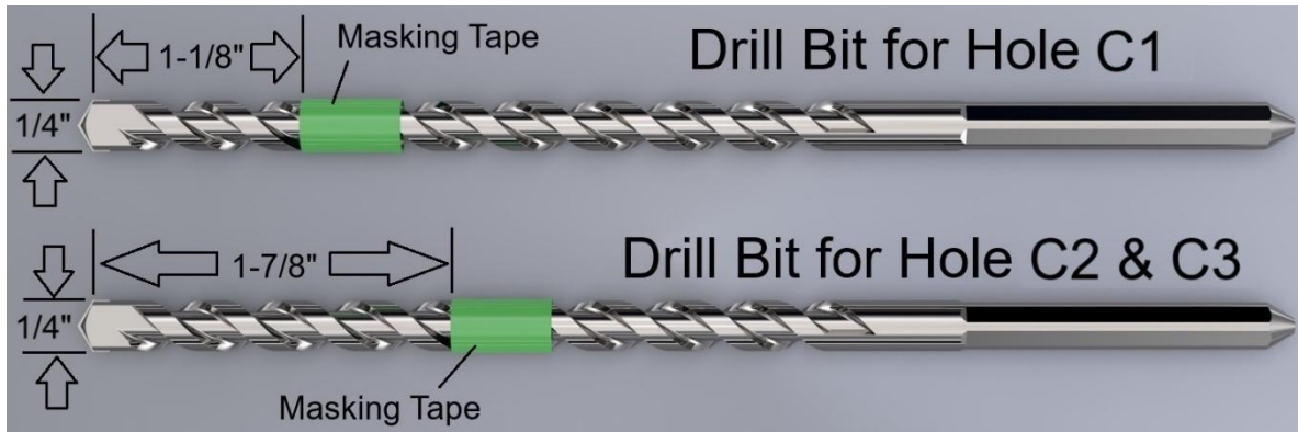
Figure 43: Masking Tape on \frac{1}{4} " Concrete Drill Bits for Holes C1, C2 & C3 for \frac{1}{4} " x 2\frac{1}{4} " long Wedge Anchor
