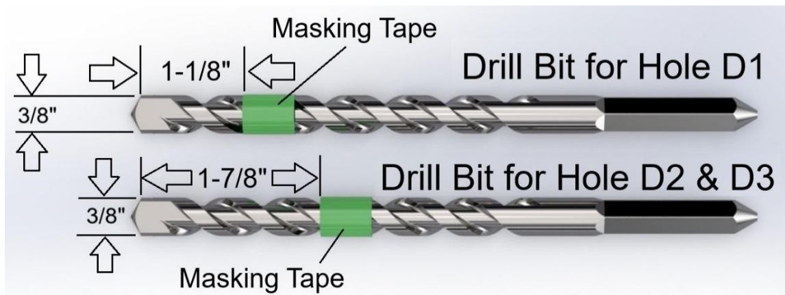
Figure 54: Masking Tape on \frac{3}{8} " Concrete Drill Bits for Holes D1, D2 & D3 for \frac{1}{4} " x 1" long Drop-In Anchors
