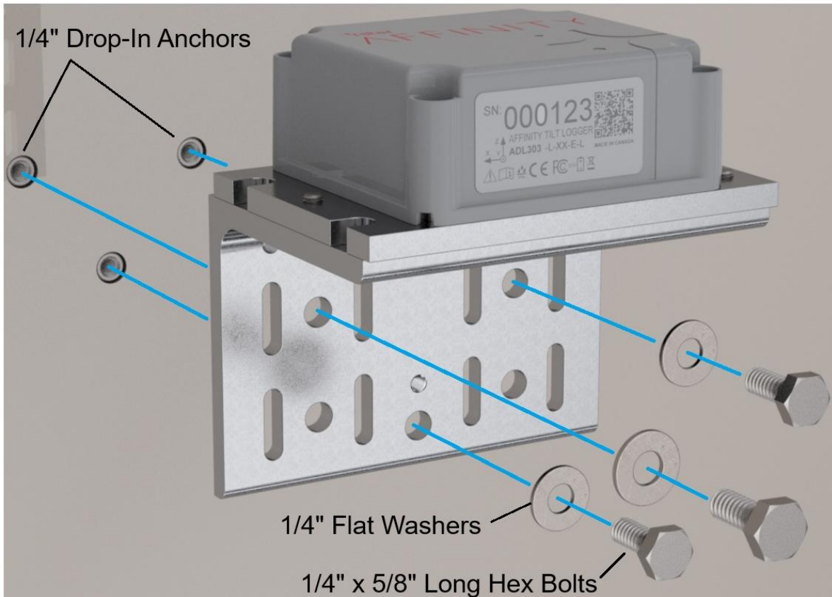
Figure 60: Installing the Affinity Tilt Logger with \frac{1}{4} " Drop-In Anchors, Hex Bolts and Washers
