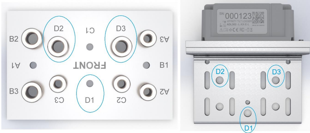
Figure 53: Drilling Template Hole Set D Corresponding to Affinity Tilt Logger Angle Bracket Mounting Holes for \frac{1}{4} " Drop-In Anchor
