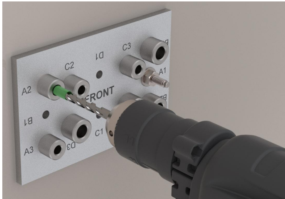
Figure 23: Drilling Second Hole Through Bushing A2 for Wedge Anchor
