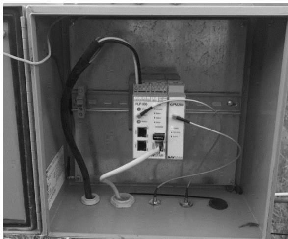
Figure 2: FLP100 with attached GPM200 module
