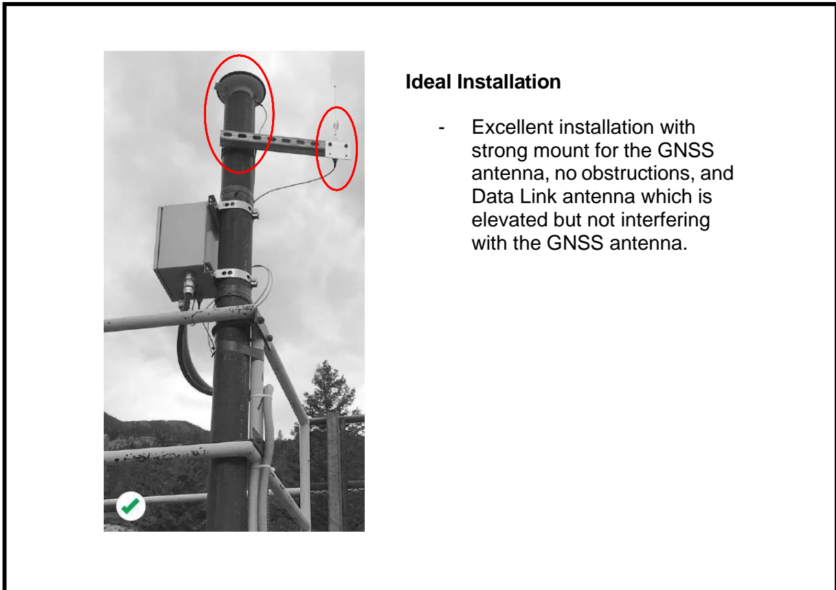
Figure 8: Example Installation
