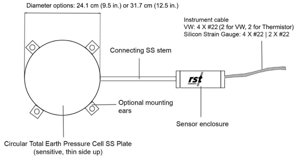
Figure 1: Total Earth Pressure Cell Diagrammatic View
