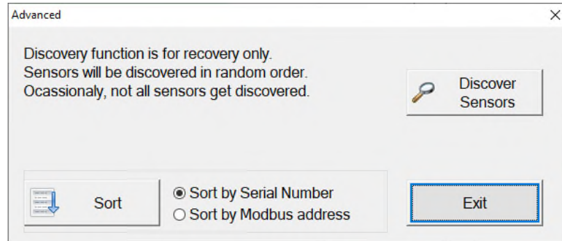
FIGURE 3-7 ADVANCED OPTIONS
