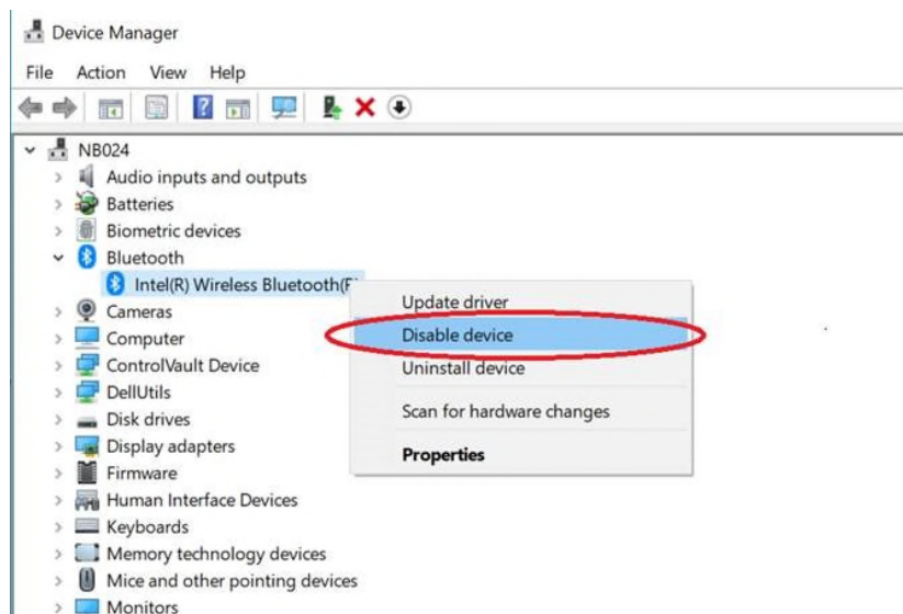
FIGURE 5-2 DISABLE BLUETOOTH
